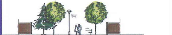
Typical Green Space/Community Trail Cross Section
