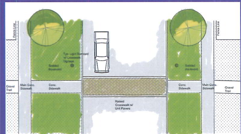
Typical Raised Crosswalk
